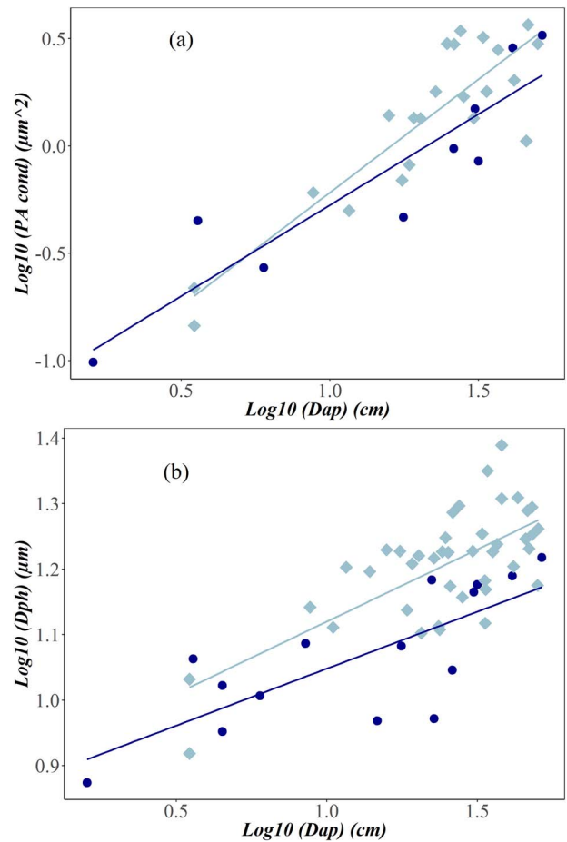
Figure 2. (a) Area of conductive phloem (PAcond) against distance from the stem apex (Dap). (b) Average diameter of the largest phloem sieve cells (Dph) for the last 5 years (after the drought of 2012) against Dap. Dark blue circles and light blue diamonds are for non-declining and declining trees, respectively.
