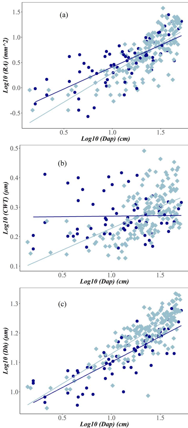
Figure 1. (a) Total ring area (RA) for the last 5 years (after the drought of 2012) against distance from the stem apex (Dap). (b) Tracheid cell wall thickness (CWT) for the last 5 years (after the drought of 2012) against Dap. Dark blue circles and light blue diamonds are for non-declining and declining trees, respectively. (c) Tracheid hydraulic diameter (Dh) for the last 5 years (after the drought of 2012) against distance from the stem apex (Dap).
